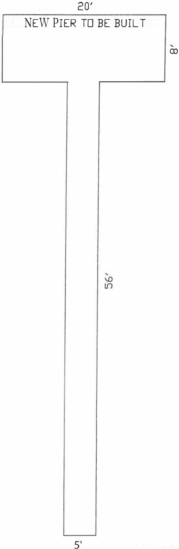
Typical Finger Pier Design
